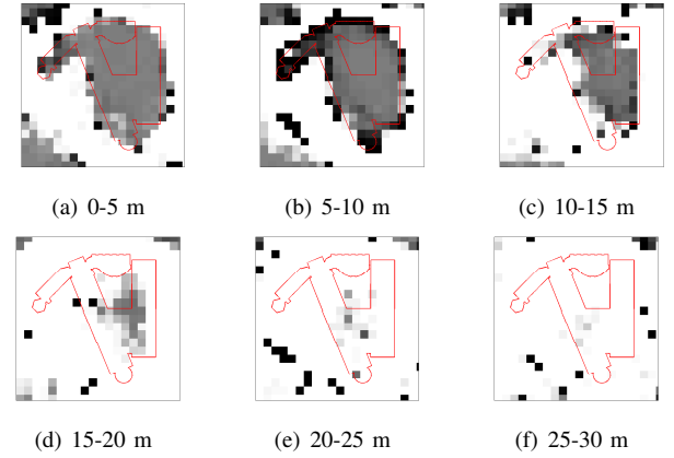
Fig. 7. Horizontal slices of the generated map around Kohn Hall at UCSB.
