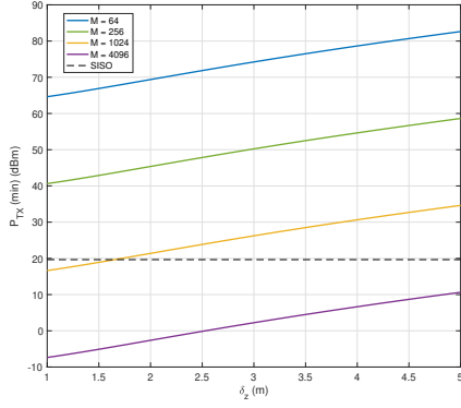
Fig. 3. P_{Tx} dBm for different RA sizes M and depth parameter \delta_z with Tx subarray size of 8 \times 8
