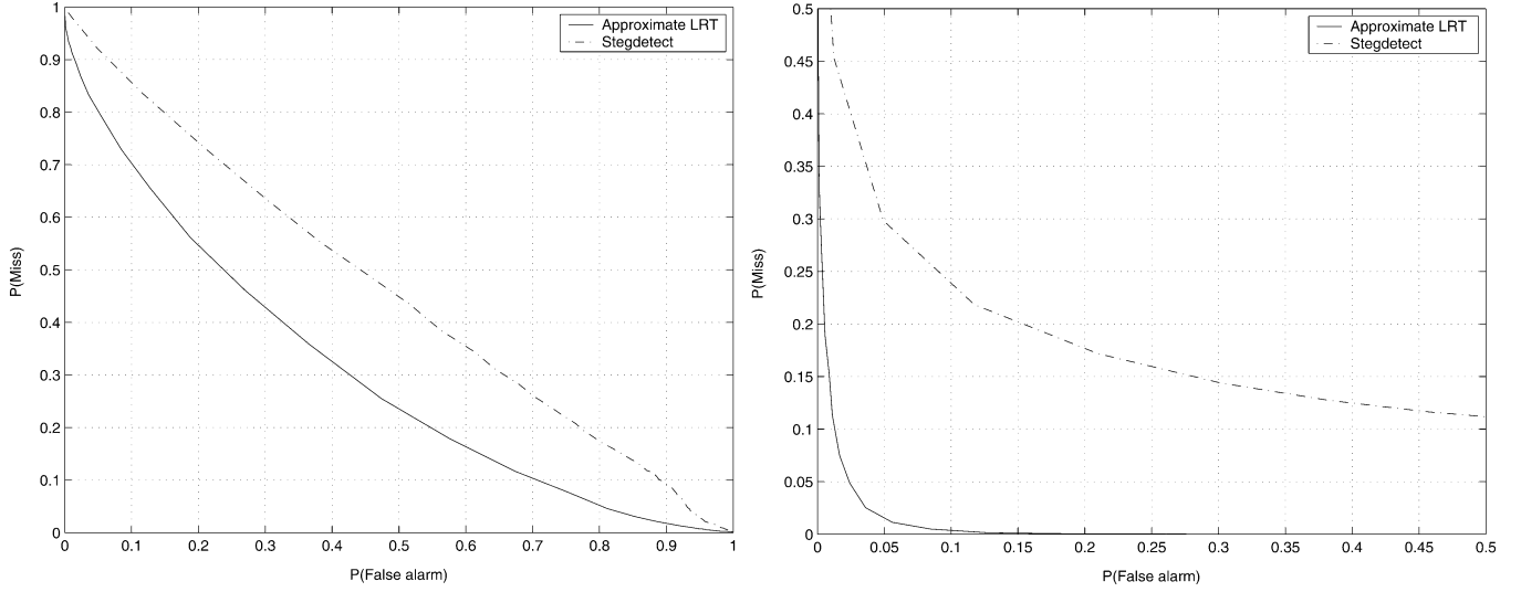
Fig. 4. Approximate LRT with half-half filter estimate versus stegdect: At high rates (right side; R = 0.5 ) as well as low rates (left side; R = 0.05 ), the approximate LRT is superior. The same hiding rate r was used for all the test images with hidden data.
