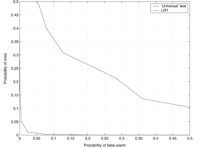
Fig. 2. Comparison between the universal test ( R_0 = 0.5 ) and the LRT test for binomial(15, 1/2) data of length 1024 and hiding rate R = 0.5 . Any practical scheme would perform between these two limits.
