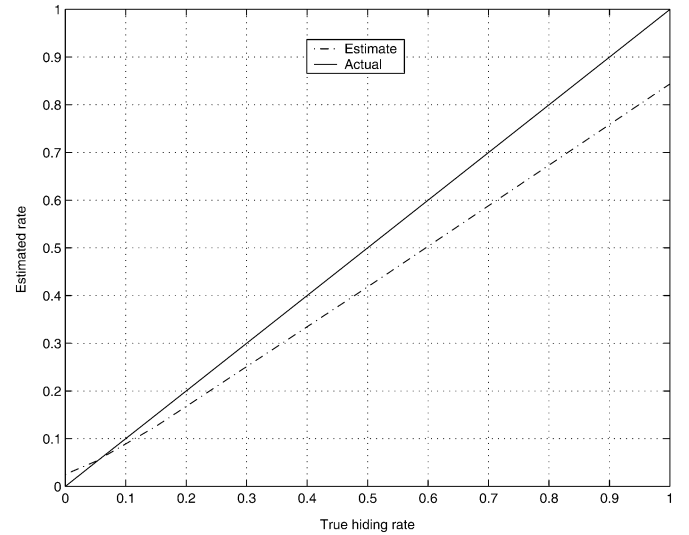
Fig. 6. Minimizing rate in (11) serves as an estimate of the true hiding rate.
