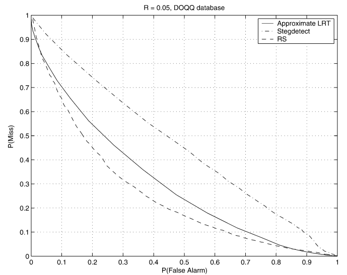
Fig. 7. RS analysis, which uses host memory, is slightly better than our memoryless approximate LRT on the DOQQ database. A hiding rate of 0.05 was used for all the test images with hidden data.
