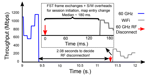
Figure 4: Temporal analysis of our platform’s FST.
